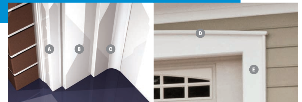
A Brick Mould B Jamb (non-load bearing) C Garage Door Stop D Drip Cap E Flat Utility Trim
